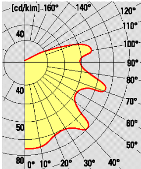
Incandescent lamp
