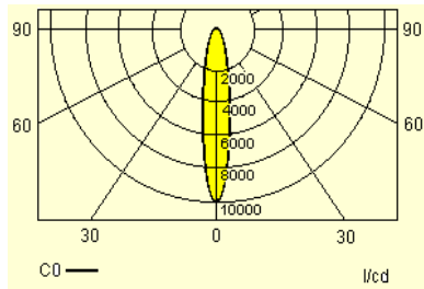
Luminous flux distribution curve
